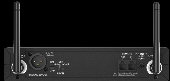
NCR1 Back Panel
