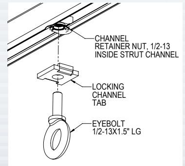
Suspension Kit
