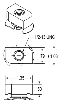
Retainer Nut
