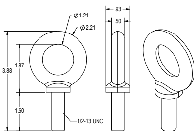
Eyebolt
