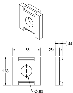
Locking Tab
