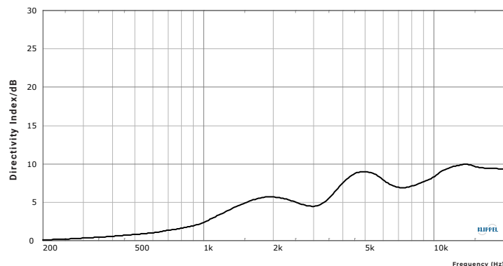
Directivity Index
