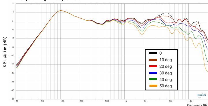
Frequency Response
