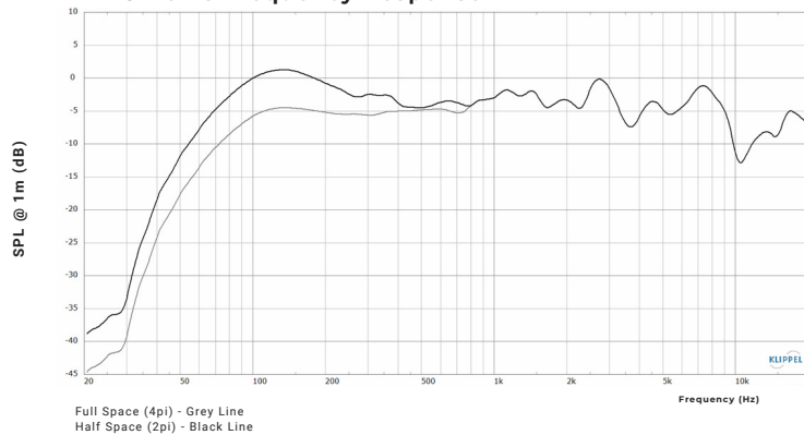
1m On-axis Frequency Response
