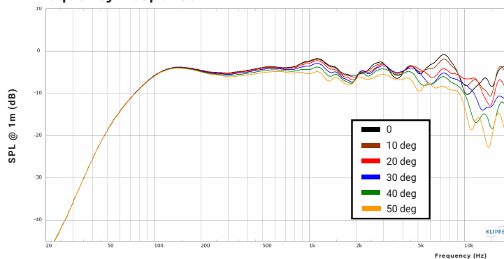
Frequency Response
