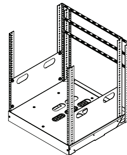
ISO VIEW
