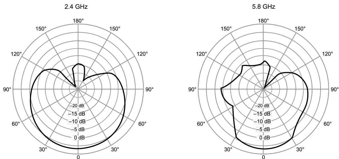
Polar Pattern
