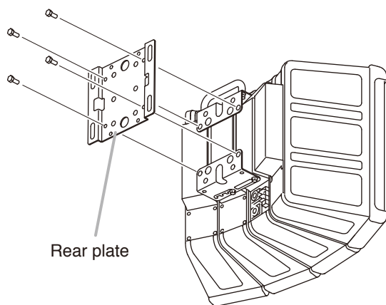
[Factory-preset mounting]
