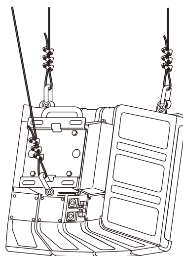
[Horizontal suspension]
