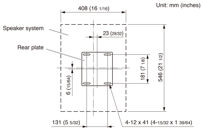
[Direct wall mounting dimensions] (Angle mode of 60°)
